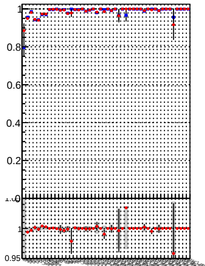
Fake rate vs. —•— DQM_DisplacedSUSY_mkFit_BDT_ —•— DQM_DisplacedSUSY_mkFit_
