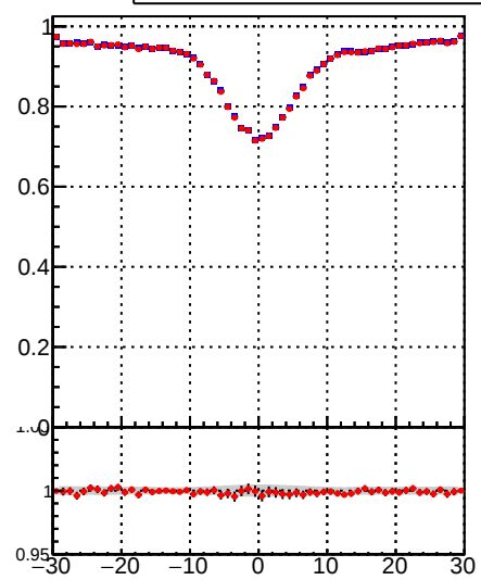
—+ DQM_DisplacedSUSY_mkFit_BDT_ —+ DQM_DisplacedSUSY_mkFit_
