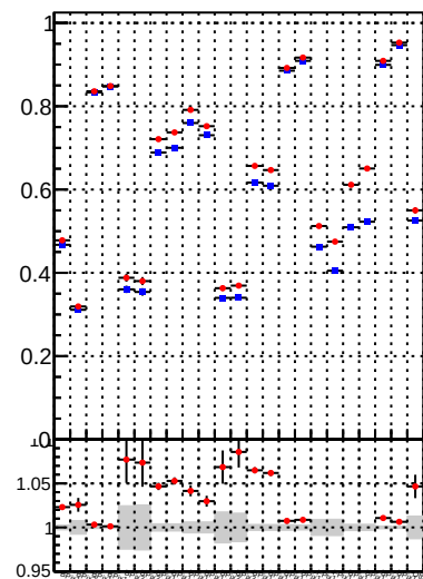
Fake rate vs. —●— DQM_DisplacedSUSY_mkFit_BDT_ —●— DQM_DisplacedSUSY_mkFit_
