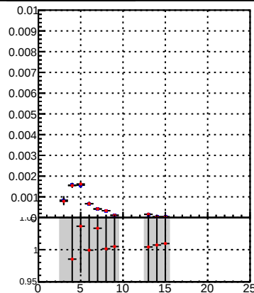
Legend: DQM_DisplacedSUSY_mkFit_BDT_ (blue line), DQM_DisplacedSUSY_mkFit_ (red line)
