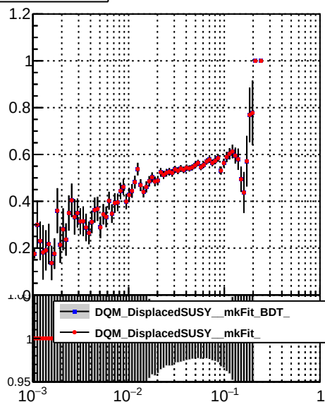
Efficiency vs \Delta R
