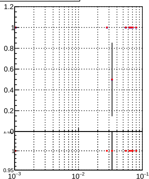
Efficiency vs \Delta R (track, jet)
