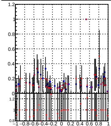
Efficiency vs DQM_DisplacedSUSY_mkFit_
