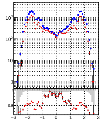
N of reco track vs \eta DQM_DisplacedSUSY_mkFit_BDT_ DQM_DisplacedSUSY_mkFit \eta eta
