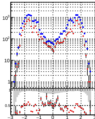
N of reco track vs \eta DQM_DisplacedSUSY_mkFit_BDT_ DQM_DisplacedSUSY_mkFit \eta eta
