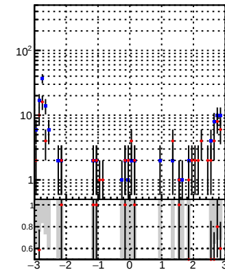
N of reco track vs \eta DQM_DisplacedSUSY_mkFit BDT_ DQM_DisplacedSUSY_mkFit \eta
