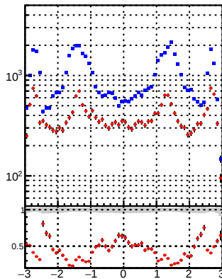
N of reco track vs \eta DQM_DisplacedSUSY_mkFit BDT_ DQM_DisplacedSUSY_mkFit \eta
