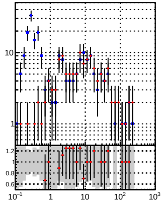
—●— DQM_DisplacedSUSY_mkFit_BDT_ —●— DQM_DisplacedSUSY_mkFit
