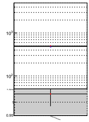
N of reco track vs. \chi^2 — DQM_DisplacedSUSY_mkFit_BDT — DQM_DisplacedSUSY_mkFit
