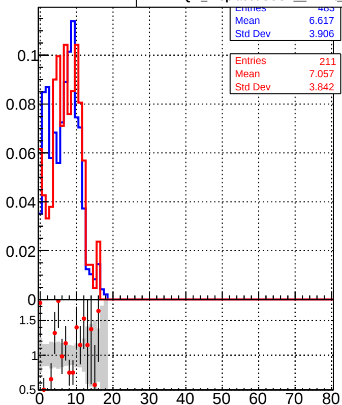
Legend: Blue line: DQM_DisplacedSUSY_mkFit_BDT_ Red line: DQM_DisplacedSUSY_mkFit_
