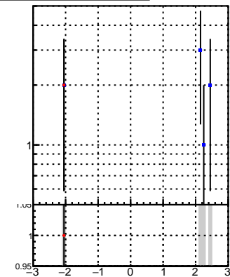
N of associated (recoToSim) tracks vs \eta —•— DQM_DisplacedSUSY_mkFit_BDT_ -+ - DQM_DisplacedSUSY_mkFit_
