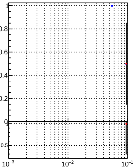
Fake rate vs \sqrt{s} DQM_DisplacedSUSY_mkFit_BDT_ DQM_DisplacedSUSY_mkFit_
