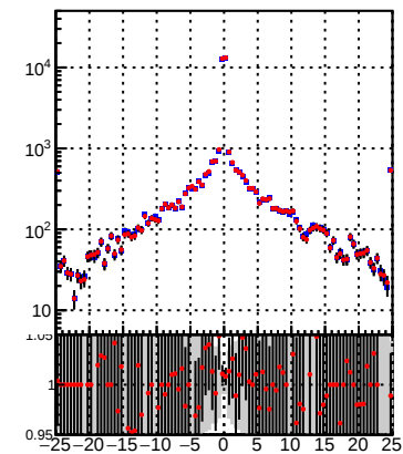
— DQM_DisplacedSUSY_mkFit_BDT_ (black line) — DQM_DisplacedSUSY_mkFit_ (red line)
