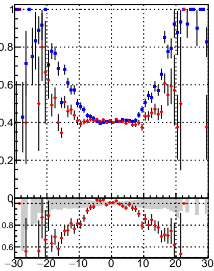
Fake rate vs \nu —■— DQM_DisplacedSUSY_mkFit_BDT —*— DQM_DisplacedSUSY_mkFit
