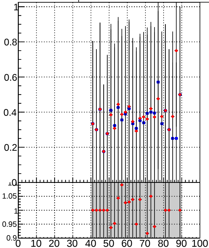
—■ DQM_DisplacedSUSY_mkFit_ —● DQM_DisplacedSUSY_mkFit_BDT_
