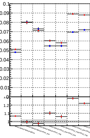
Fake rate vs. —•— DQM_DisplacedSUSY_mkFit —•— DQM_DisplacedSUSY_mkFit_BDT
