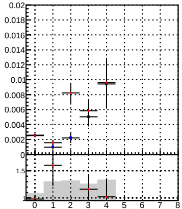
Duplicates Rate vs pixel layer
