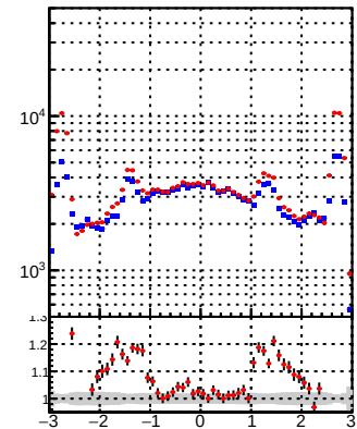
N of reco track vs \eta DQM_DisplacedSUSY_mkFit DQM_DisplacedSUSY_mkFit_BDT
