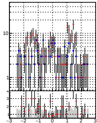
N of reco track vs \eta DQM_DisplacedSUSY_mkFit DQM_DisplacedSUSY_mkFit_BDT
