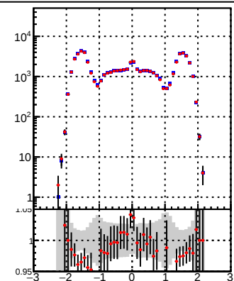
dSUSY mkFit BDT
