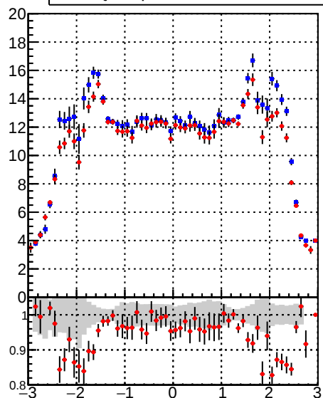
mean hit — DQM_DisplacedSUSY_mkFit_ — DQM_DisplacedSUSY_mkFit_BDT_
