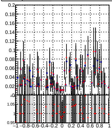
Efficiency vs Dxy(PV) Legend: DQM_DisplacedSUSY_mkFit_ (blue squares) DQM_DisplacedSUSY_mkFit_BDT_ (red circles)
