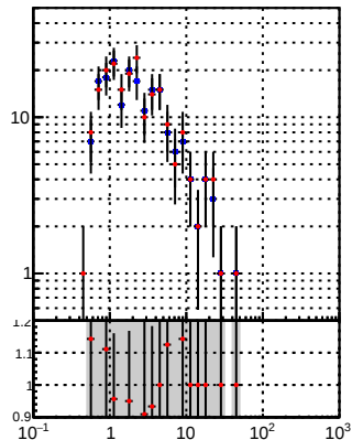
—•— DQM_DisplacedSUSY_mkFit —•— DQM_DisplacedSUSY_mkFit_BDT
