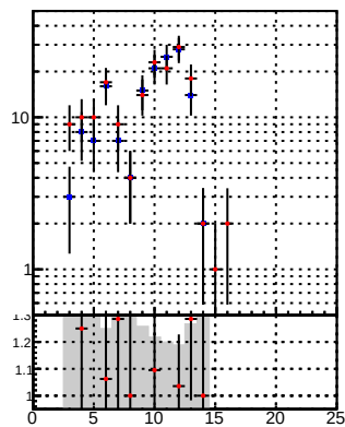
edSUSY__mkFit_BDT_
