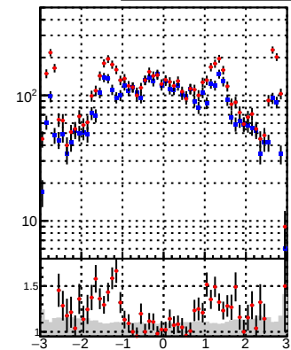
N of reco track vs \eta Legend: DQM_DisplacedSUSY_mkFit DQM_DisplacedSUSY_mkFit_BDT_
