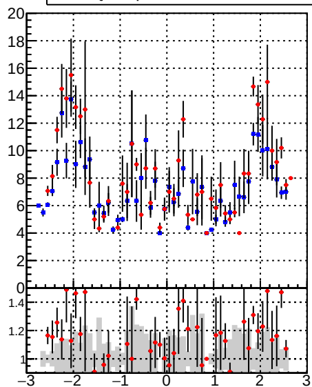
mean hit Legend: DQM_DisplacedSUSY_mkFit_ (Blue line), DQM_DisplacedSUSY_mkFit_BDT_ (Red line)
