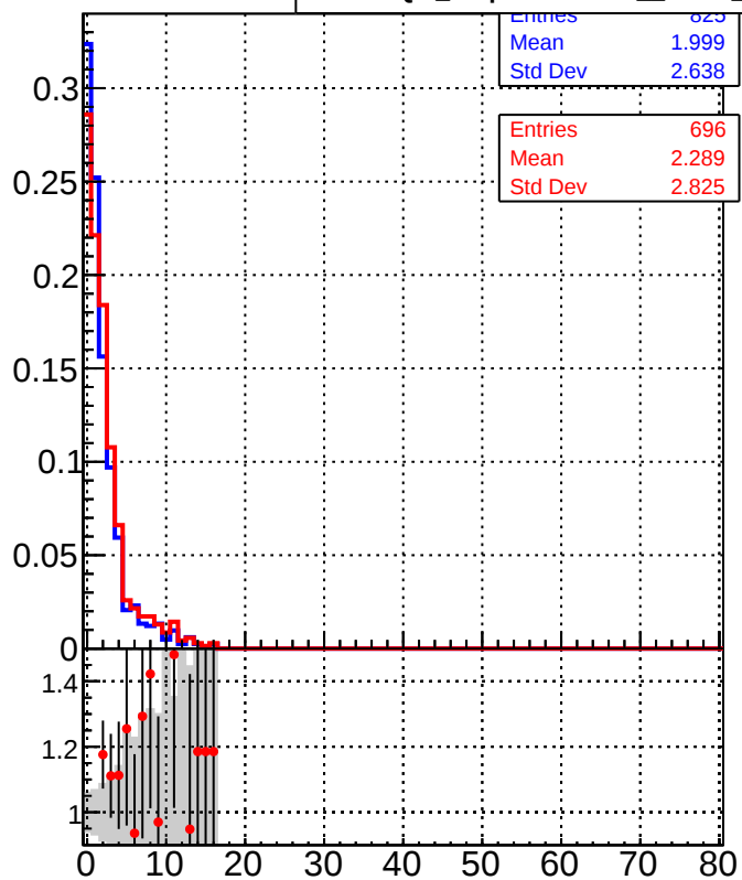
Legend: QGM_DisplacedSUSY_mkFit_ (Blue line with squares) QGM_DisplacedSUSY_mkFit_BDT_ (Red line with circles)
