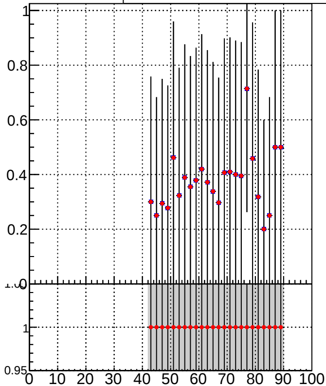
—■— DQM_DisplacedSUSY_mkFit_ —●— DQM_DisplacedSUSY_mkFit_BDT_
