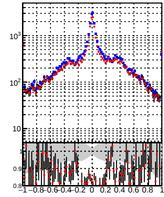
N of reco track vs d
