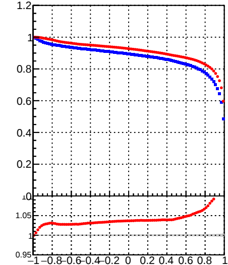
Efficiency (tracking eff factorized out) vs. MVA1
