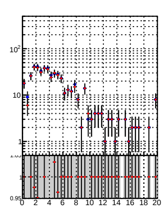
N of reco track vs. \chi^2 DQM_DisplacedSUSY_mkFit DQM_DisplacedSUSY_mkFit_BDT_
