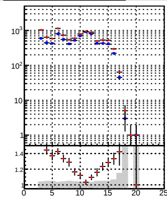
edSUSY__mkFit_BDT_
