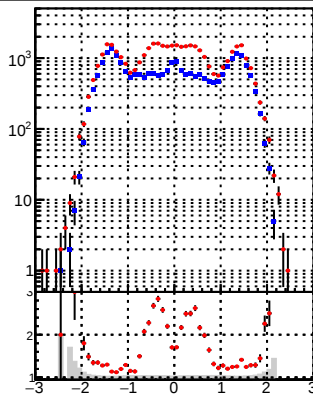
N of reco track vs \eta DQM_DisplacedSUSY_mkFit DQM_DisplacedSUSY_mkFit_BDT \eta
