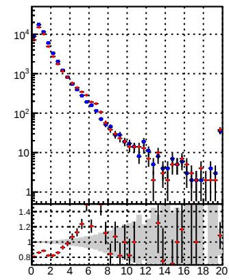
N of reco track vs. \chi^2 DQM_DisplacedSUSY_mkFit DQM_DisplacedSUSY_mkFit_BDT
