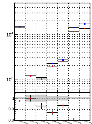
N of reco track vs. \chi^2 DQM_DisplacedSUSY_mkFit DQM_DisplacedSUSY_mkFit_BDT
