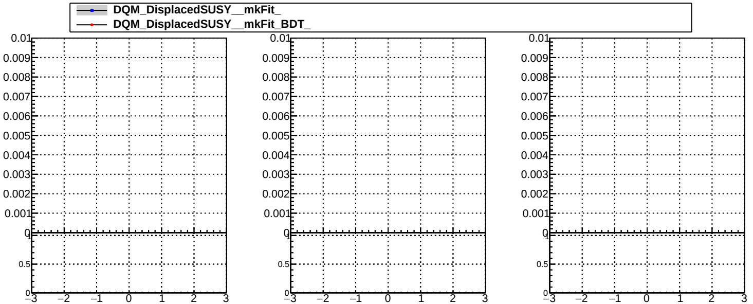
Fake rate vs \phi
