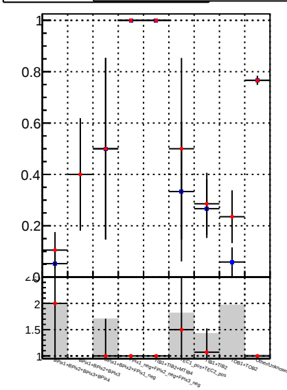
Fake rate vs. —•— DQM_DisplacedSUSY_mkFit —•— DQM_DisplacedSUSY_mkFit_BDT
