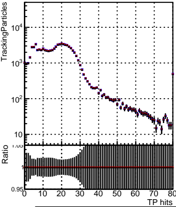
Legend for TrackingParticles vs TP hits: DQM_V0001_R000000001_Global_cmsswQCD_RECO (Blue line with squares) DQM_V0001_R000000001_Global_mkFitOriginalQCD_RECO (Red line with circles) DQM_V0001_R000000001_Global_mkFitNewQCD_RECO (Black line with crosses)
