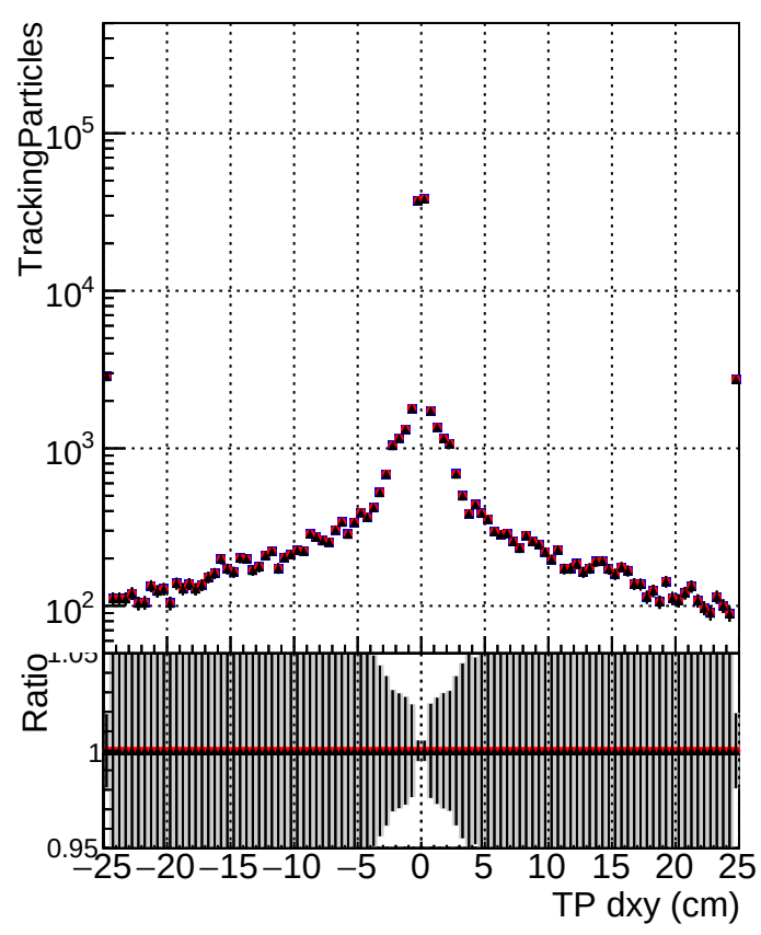
N of simulated track ■ DQM_V0001_R000000001 Global cmsswQCD RECO ● DQM_V0001_R000000001 Global mkFitOriginalQCD RECO ▲ DQM_V0001_R000000001 Global mkFitNewQCD RECO
