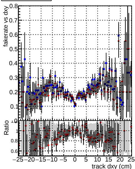
DOM V0001 R0000000001 Global cmsNewQCD RECO DOM V0001 R0000000001 Global mktNewQCD RECO
