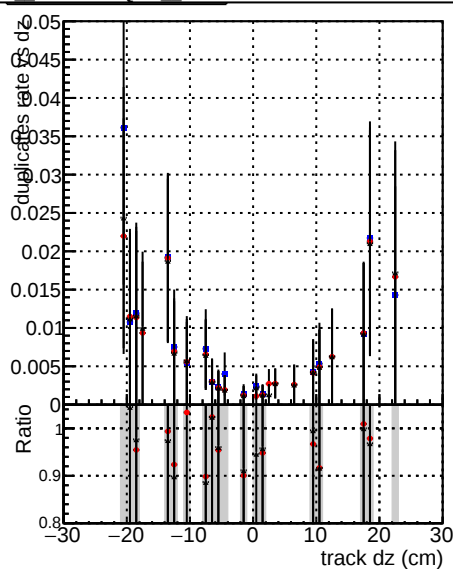
DOM V0001 R0000000001 Global cmsNewQCD RECO DOM V0001 R0000000001 Global mktNewQCD RECO
