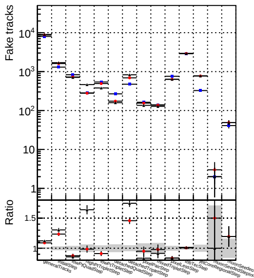
Number ● DQM_V0001_R0000000001_Global_mkFitOriginalQCD_RECO ★ DQM_V0001_R0000000001_Global_mkFitNewQCD_RECO
