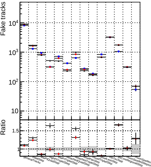
Number Legend DQM_V0001_R0000000001_Global_mkFitOriginalQCD_RECO DQM_V0001_R0000000001_Global_mkFitNewQCD_RECO
