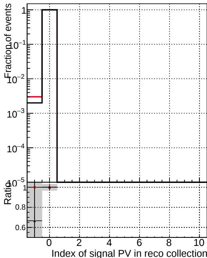
TruePVLocationIndexInRecoVertexCollection
