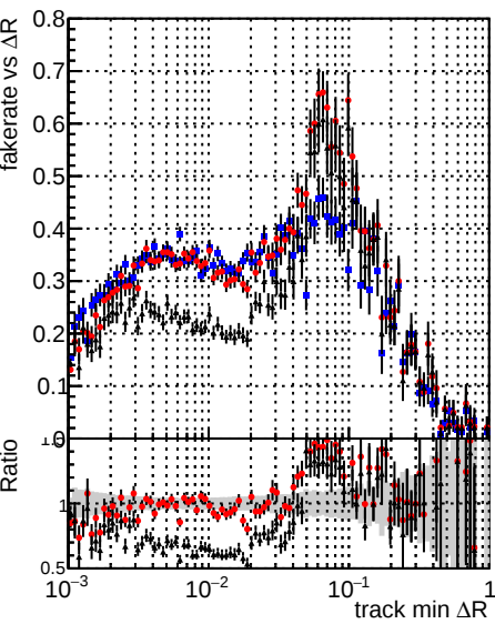
Legend: DQM_V0001_R000000001 Global_cmsswQCD_RECO, DQM_V0001_R000000001 Global_mkFitOriginalQCD_RECO, DQM_V0001_R000000001 Global_mkFitNewQCD_RECO
