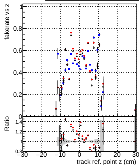
Legend for all plots: —•— DQM_V0001_R000000001 Global cmsswQCD_RECO —•— DQM_V0001_R000000001 Global mkFitOriginalQCD_RECO —•— DQM_V0001_R000000001 Global mkFitNewQCD_RECO
