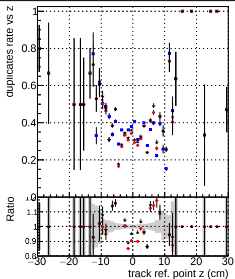
Legend for all plots: —•— DQM_V0001_R000000001 Global cmsswQCD_RECO —•— DQM_V0001_R000000001 Global mkFitOriginalQCD_RECO —•— DQM_V0001_R000000001 Global mkFitNewQCD_RECO
