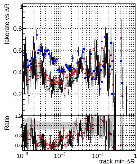
—●— DQM_V0001_R000000001_Global_cmsswQCD_RECO —●— DQM_V0001_R000000001_Global_mkFitOriginalQCD_RECO —●— DQM_V0001_R000000001_Global_mkFitNewQCD_RECO
