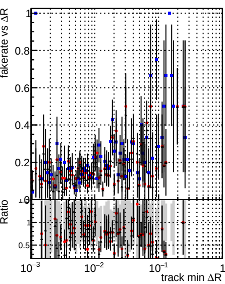
Fake rate vs \Delta R(\text{track, jet}) DQM_V0001_R000000001 Global cmsswQCD_RECO DQM_V0001_R000000001 Global mkFitOriginalQCD_RECO DQM_V0001_R000000001 Global mkFitNewQCD_RECO
