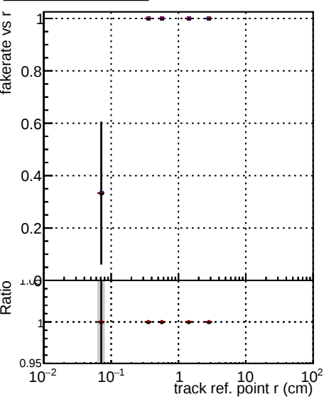
Legend: DQM_V0001_R0000000001 Global cmsswQCD RECO, DQM_V0001_R0000000001 Global mkFitOriginalQCD RECO, DQM_V0001_R0000000001 Global mkFitNewQCD RECO
