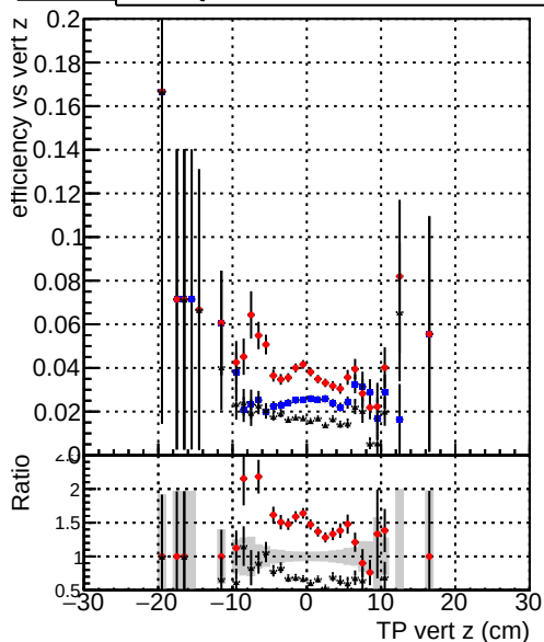
—●— DQM_V0001_R000000001_Global_cmsswQCD_RECO —●— DQM_V0001_R000000001_Global_mkFitOriginalQCD_RECO —●— DQM_V0001_R000000001_Global_mkFitNewQCD_RECO
