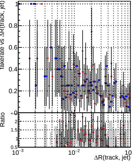
Fake rate vs \Delta R(\text{track, jet}) Legend: Global cmsswQCD_RECO (blue squares) Global mkFitOriginalQCD_RECO (red circles) Global mkFitNewQCD_RECO (black circles)
